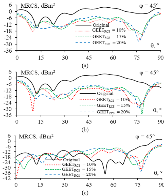
Fig. 9. Simulated total (a, d), cross-pol (b, e), and co-pol (c, f) MRCSs at 6 GHz when the structures were excited by the RHCP plane wave for the original and sparse antennas after L-RCS-OCGA
