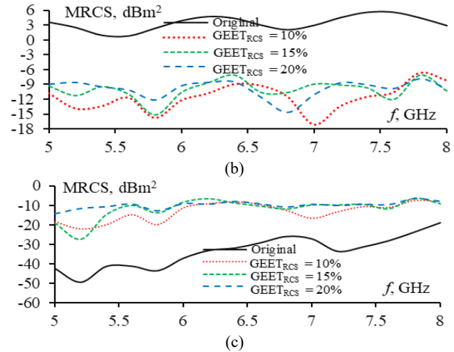
Fig. 8. Simulated total (a), cross-pol (b), and co-pol (c) MRCSs over 5-8 GHz when the structures were excited by the RHCP plane wave for the original and sparse antennas after L-RCS-OCGA
