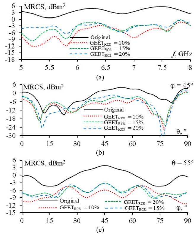
Fig. 7. Simulated MRCSs when the structures were excited by the plane wave with \theta -pol over 5–8 GHz (a), in \phi = 45^\circ (b), \theta = 55^\circ (c) planes at 6 GHz for the original and sparse antennas
