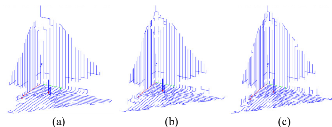
Fig. 5. Sparse antennas after L-RCS-OCGA with GEET_{RCS} = 10\% (a), 15% (b), and 20% (c)
