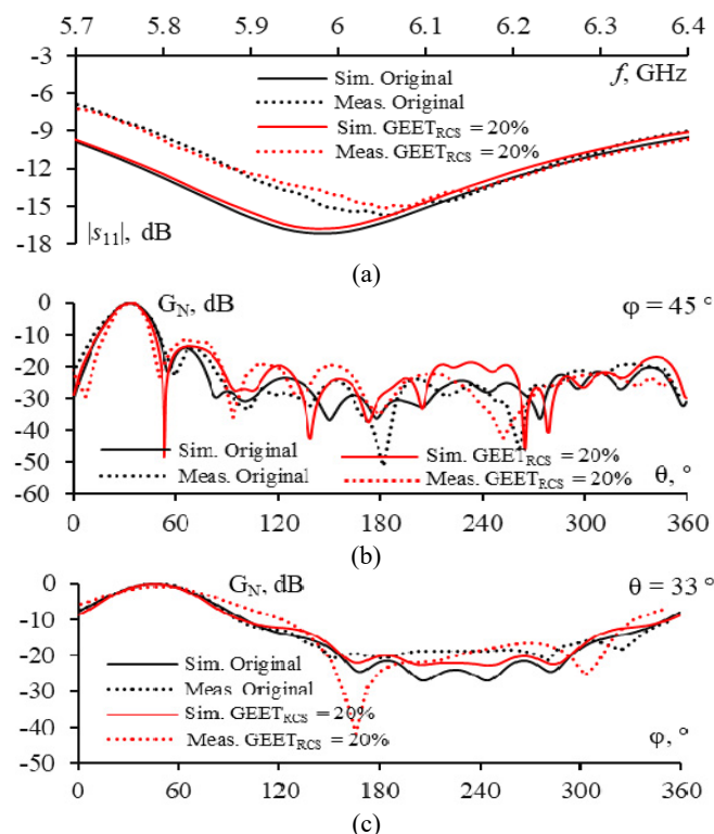
Fig. 11. Simulated and measured results of |s_{11}| (a) and RPs in the \varphi = 45^\circ (b), \theta = 33^\circ (c) planes at 6 GHz for the original and sparse antennas
