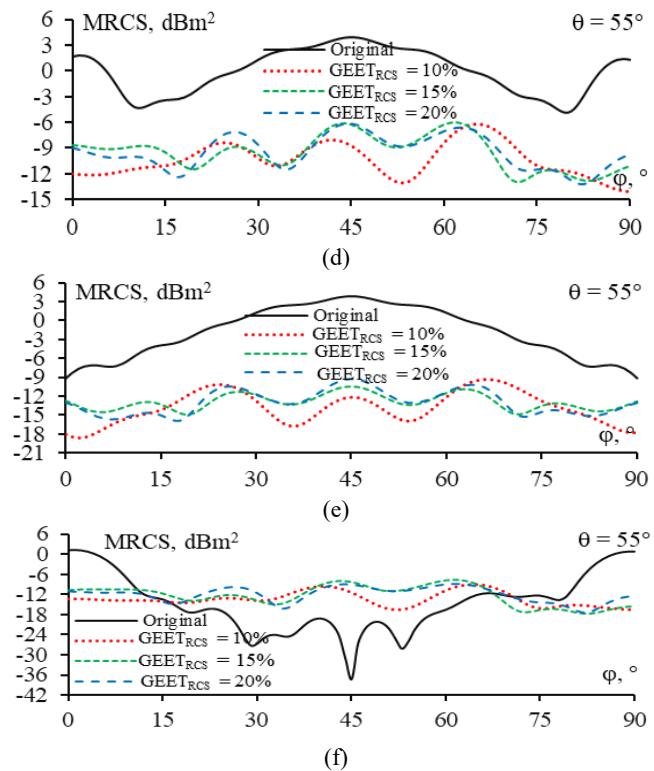
Fig. 9. Simulated total (a, d), cross-pol (b, e), and co-pol (c, f) MRCSs at 6 GHz when the structures were excited by the RHCP plane wave for the original and sparse antennas after L-RCS-OCGA
